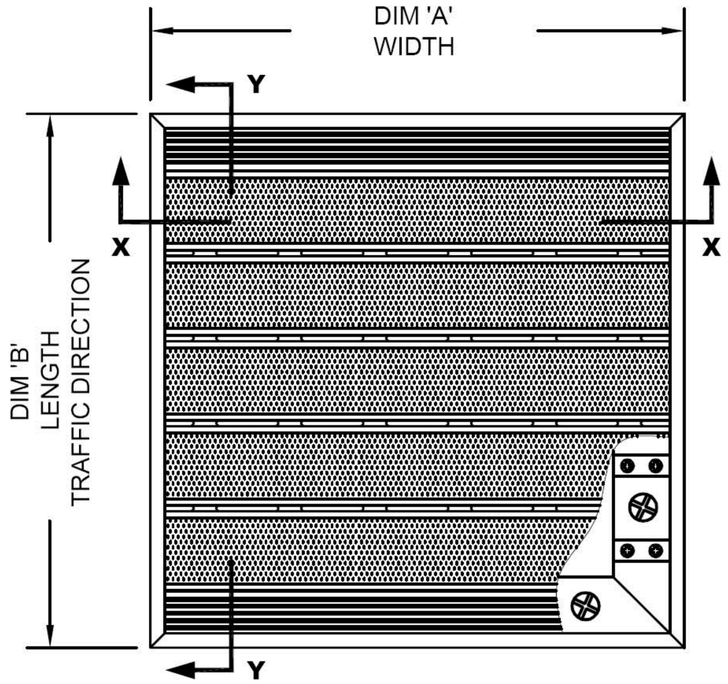
TYPICAL PLAN VIEW
